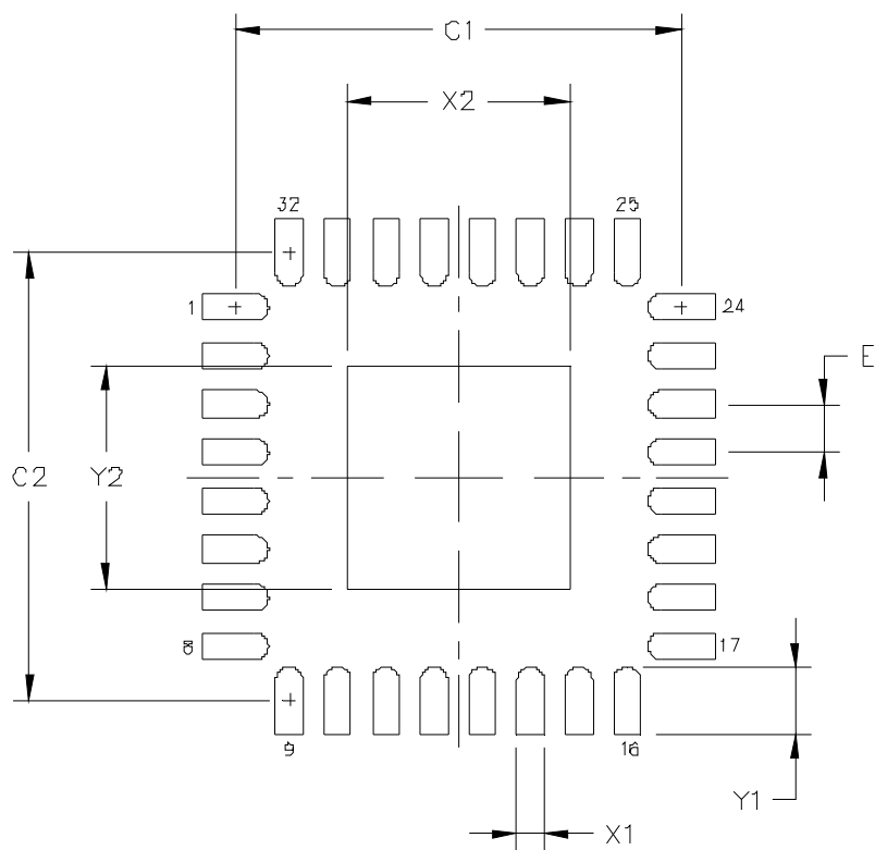
Figure 16. Si53325 32-QFN Package Land Pattern
