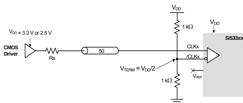
Figure 3. LVCMOS DC-Coupled Input Termination
