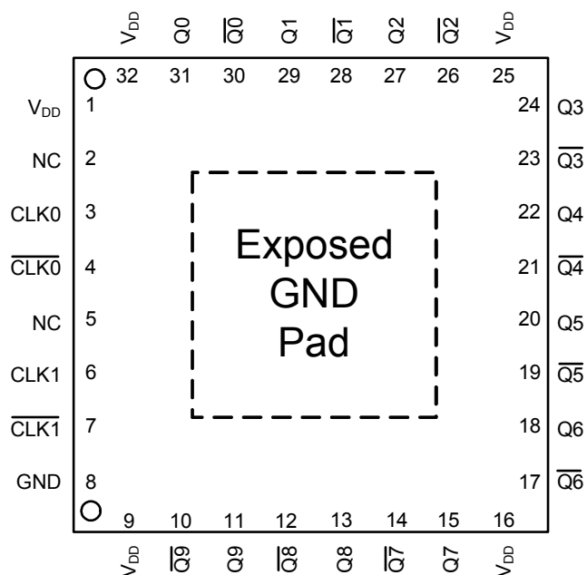
Figure 12. 32-QFN Pin Diagram (Top View)
