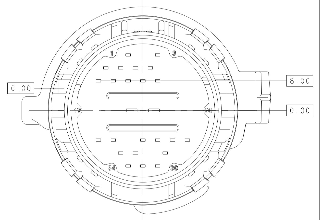
SCALE 2:1 1-2356151-1 KEYING OPTION "A", 25P DE-POPULATION
