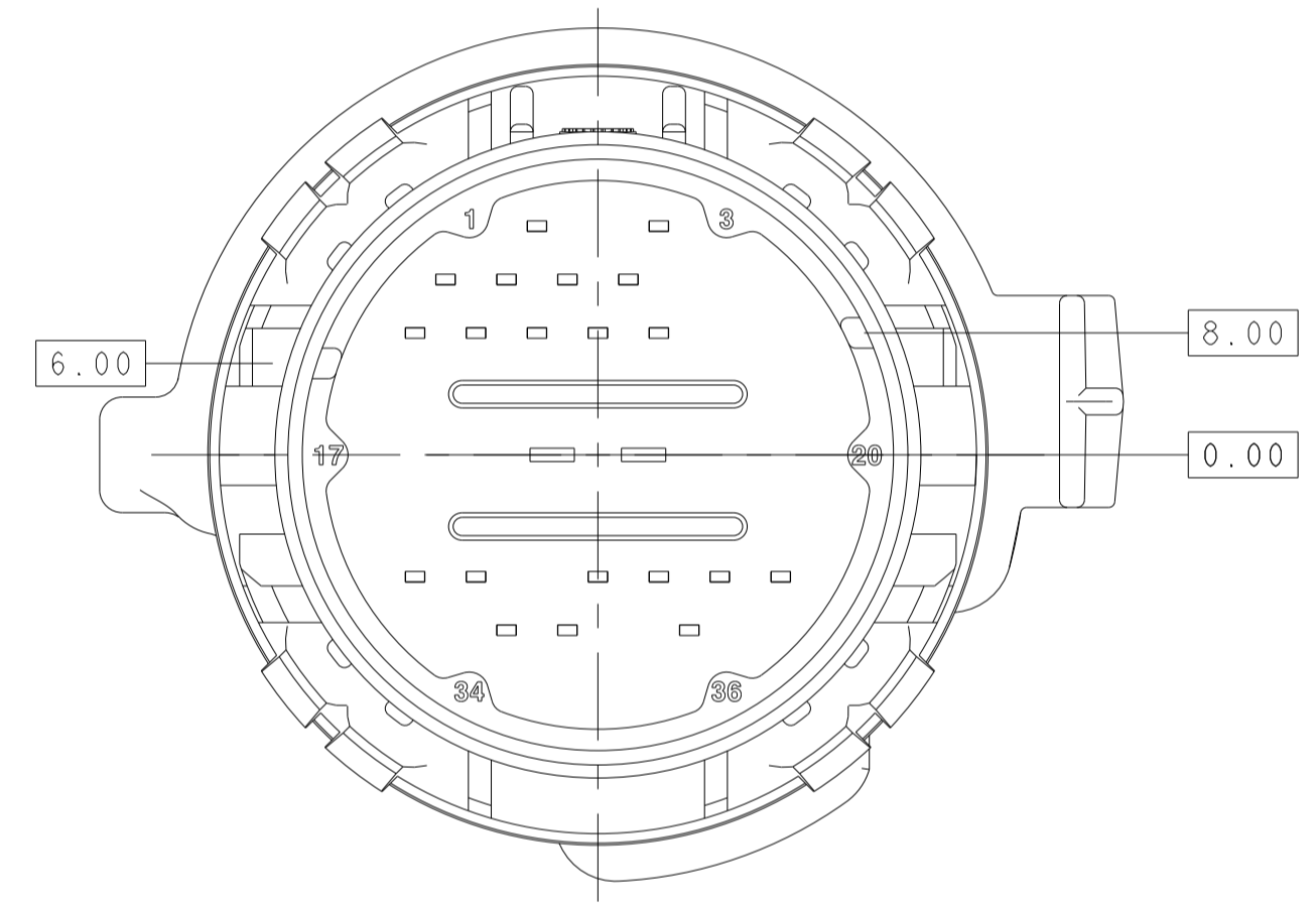
SCALE 2:1 1-2356151-0 KEYING OPTION "A", 22P DE-POPULATION
