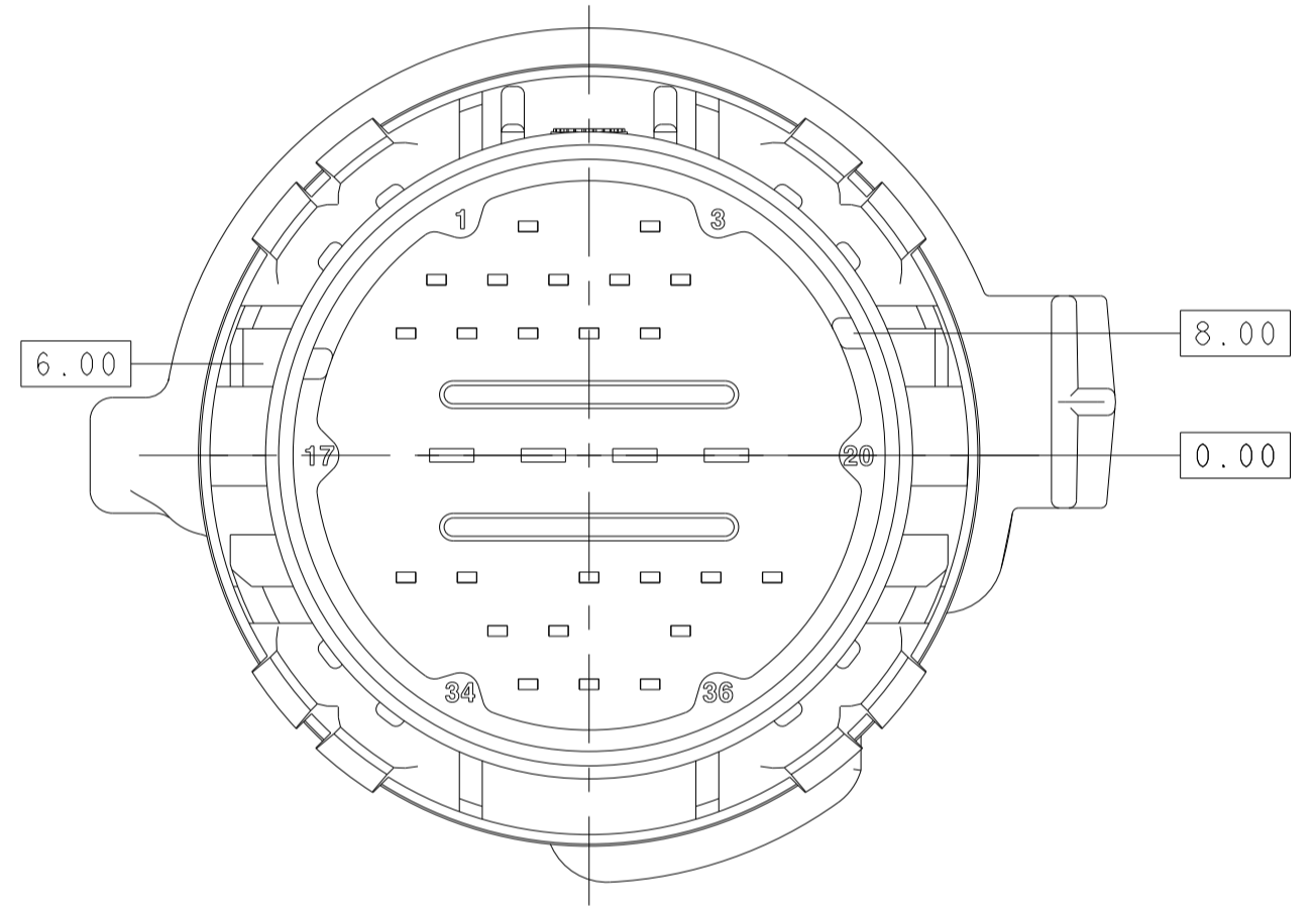
SCALE 2:1 2356151-9 KEYING OPTION "A", 28P DE-POPULATION
