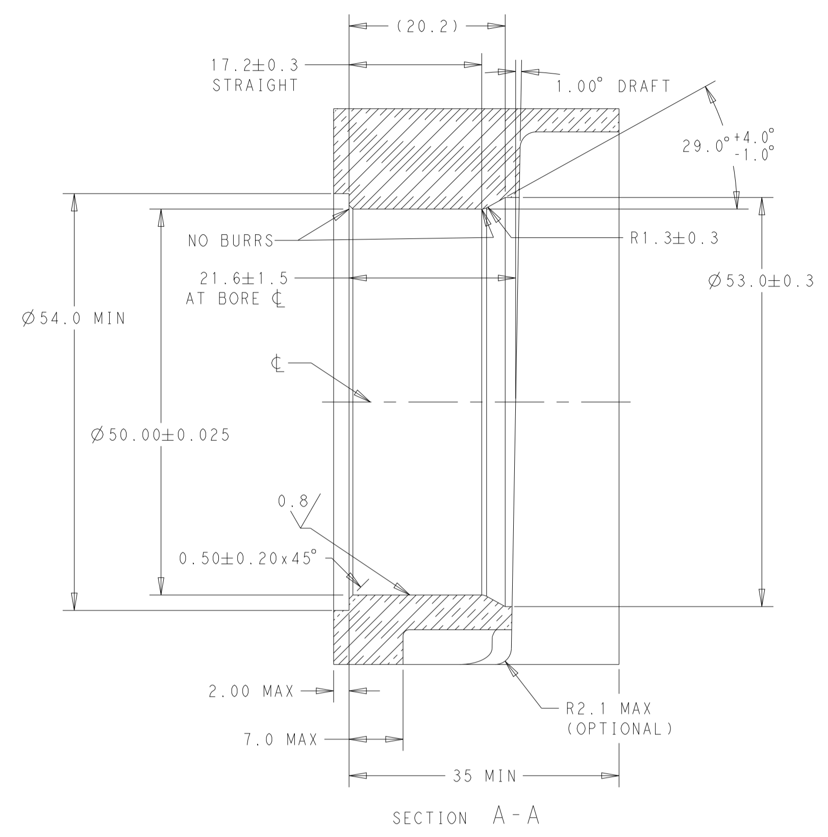
RECOMMENDED MOUNTING HOLE DETAIL
