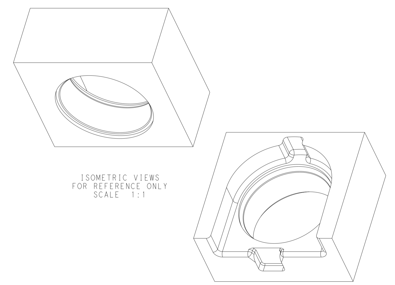
RECOMMENDED MOUNTING HOLE DETAIL
