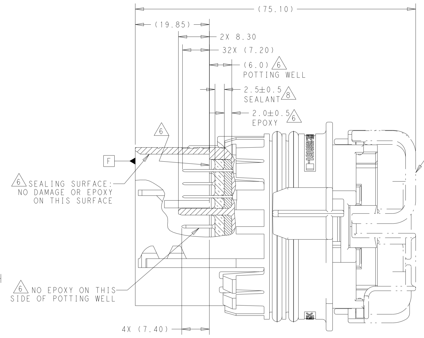
SECTION B-B
