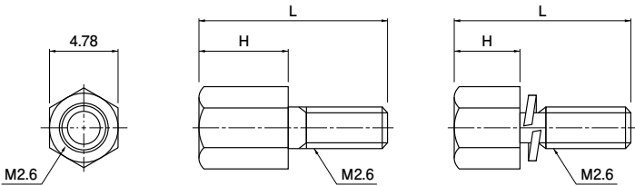
Type A Type B Hexagonal lock screw & spring washer are integrated
