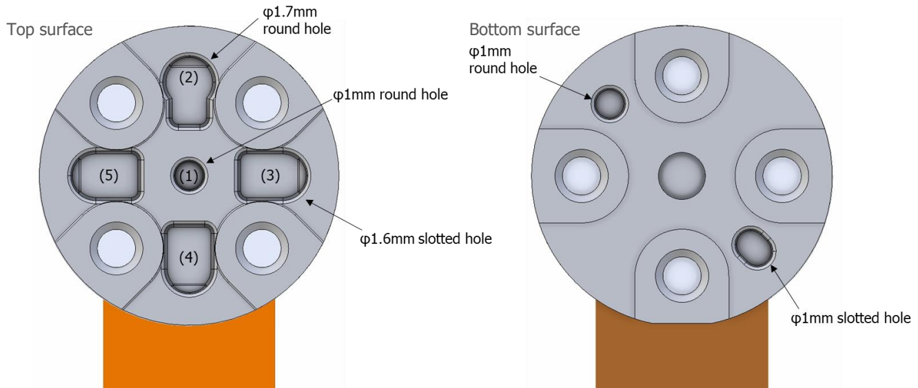
Fig. 35 Positioning holes
