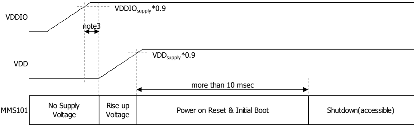
Fig. 5 Power-on sequence
