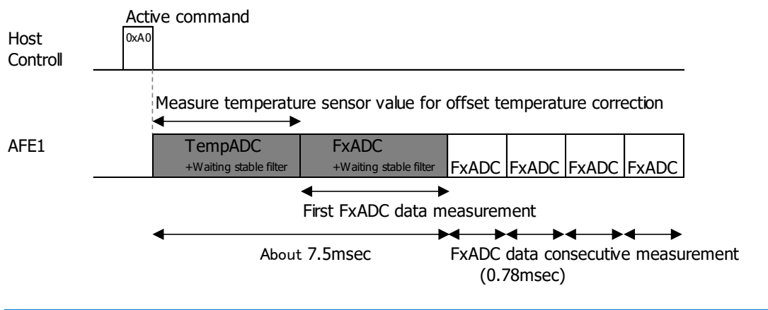
Fig. 12 Schematic of AD conversion start instruction
