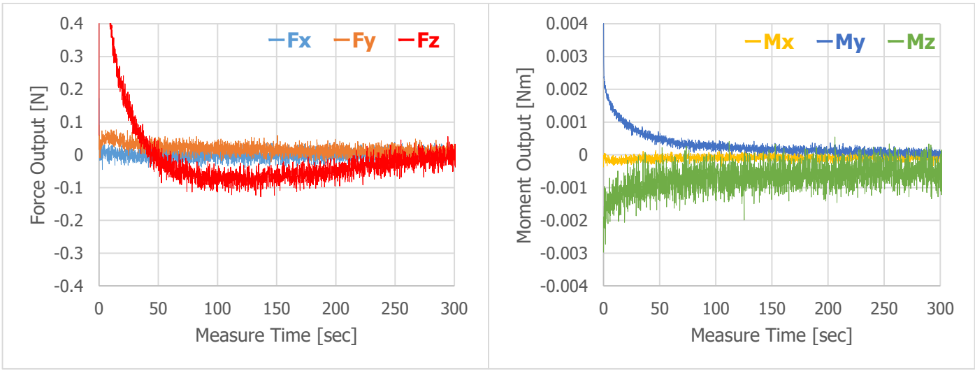
Fig. 13 Outputting data immediately after AD conversion starts
