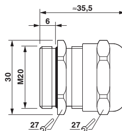
Dimensional drawing
