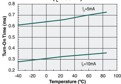
Turn-On Time vs. Temperature ( I_L=100\text{mA} )
