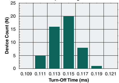
Typical Turn-Off Time Distribution (N=50, I_F=5\text{mA} , I_L=100\text{mA} )
