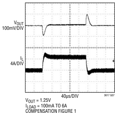
Load Step Transient
