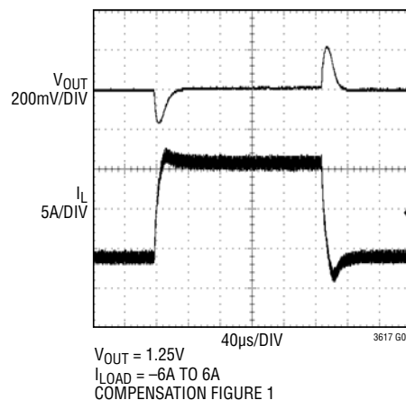
Load Step Transient
