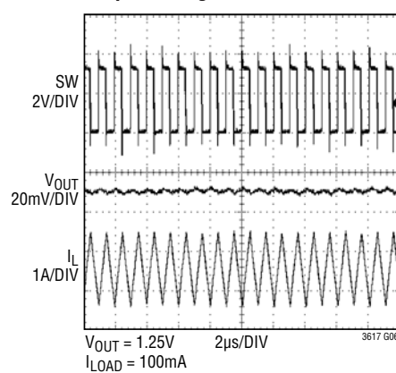
Output Voltage vs Time
