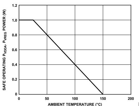
Figure 3. Thermal Derivative Curve, Dependence of Safety Limiting Values with Ambient Temperature per DIN VDE V 0884-10
