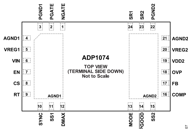
Figure 5. 24-Terminal LGA Pin Configuration
