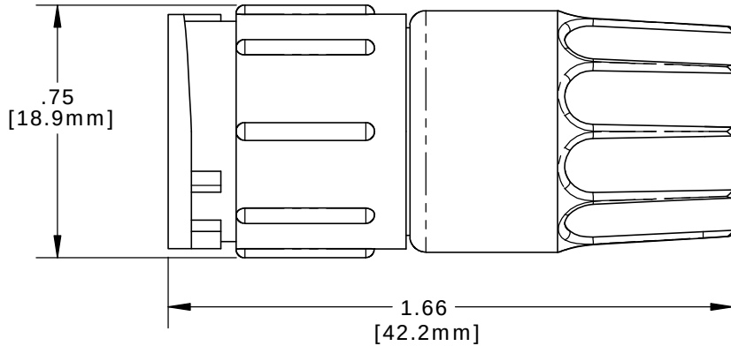
ASSEMBLED VIEW
