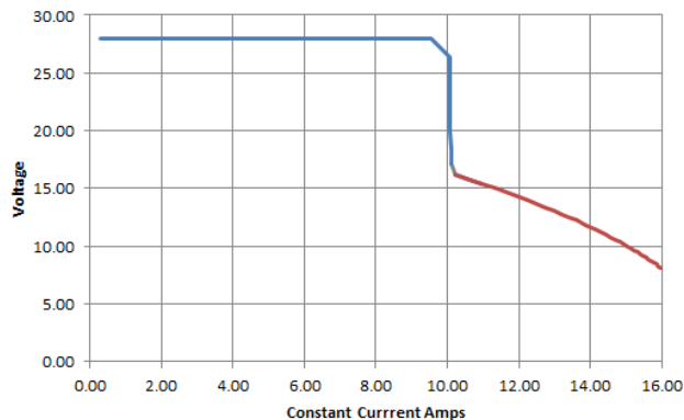
PQC250-28C Constant Current Performance
