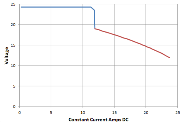
PQC250-24C Constant Current Performance
