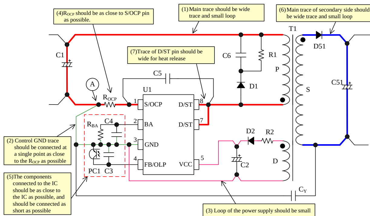
Figure 10-5. Peripheral Circuit Example Around IC
