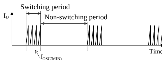
Figure 9-12. Switching Waveform at Burst Oscillation
