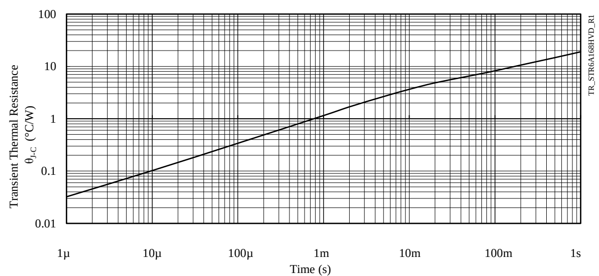
Figure 3-11. STR6A168HV/HVD Transient Thermal Resistance Curve
