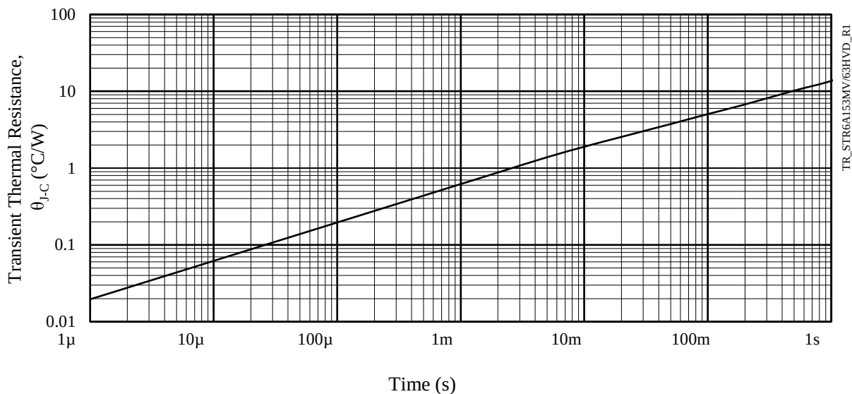
Figure 3-8. STR6A153MV and STR6A153MVD Transient Thermal Resistance Curve
