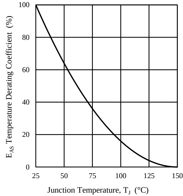
Figure 3-2. Avalanche Energy Derating Coefficient Curve
