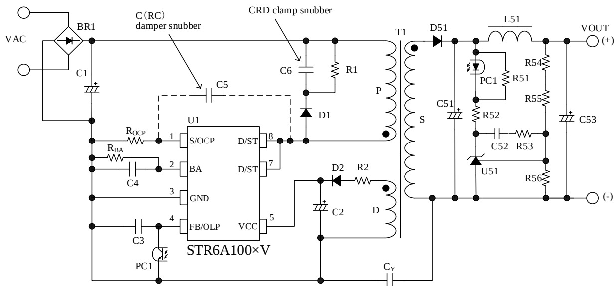
Figure 6-1. Typical Application
