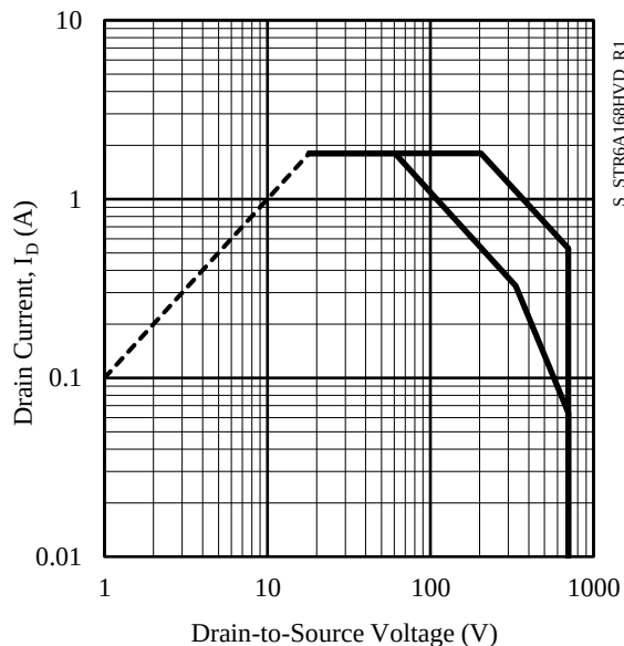
Figure 3-7. STR6A168HV/HVD SOA Curve
