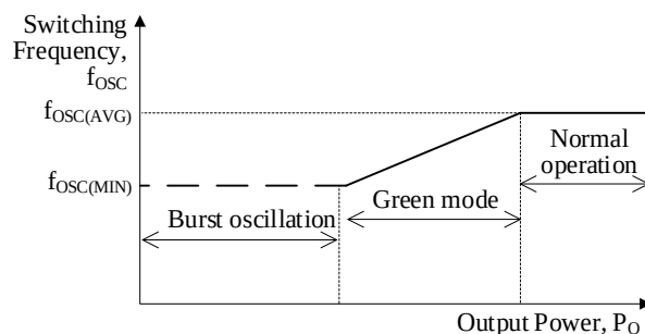
Figure 9-11. Relationship between P_O and f_{OSC}
