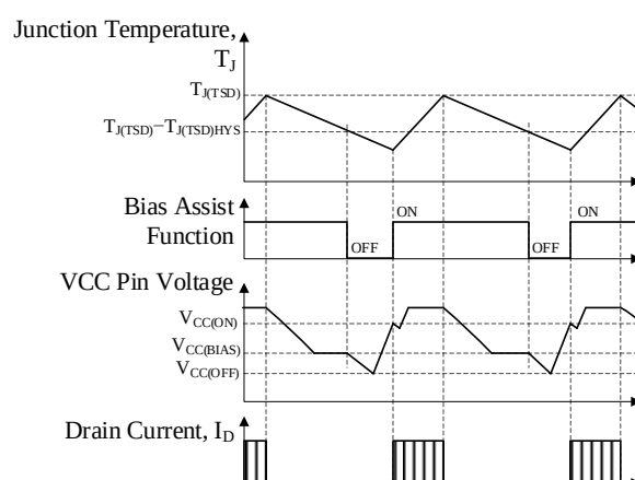
Figure 9-20. TSD Operational Waveforms (Auto-restart)
