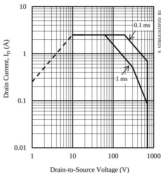
Figure 3-5. STR6A161HV/HVD SOA Curve
