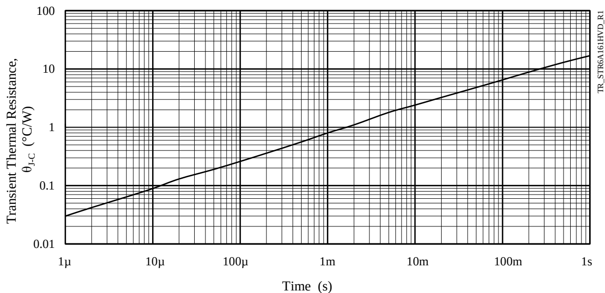
Figure 3-9. STR6A161HV/HVD Transient Thermal Resistance Curve
