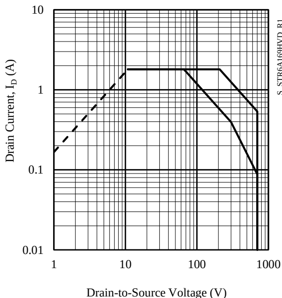
Figure 3-6. STR6A169HVD SOA Curve
