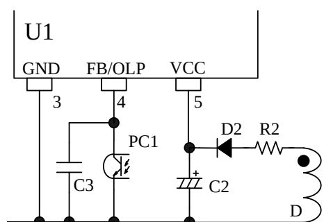
Figure 9-17. FB/OLP Pin Peripheral Circuit
