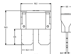
Dimensions [mm]
