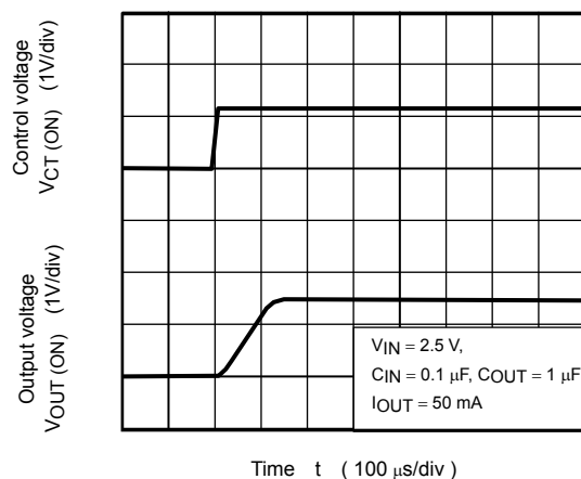
TCR5SB15A (Turn on wave form)
