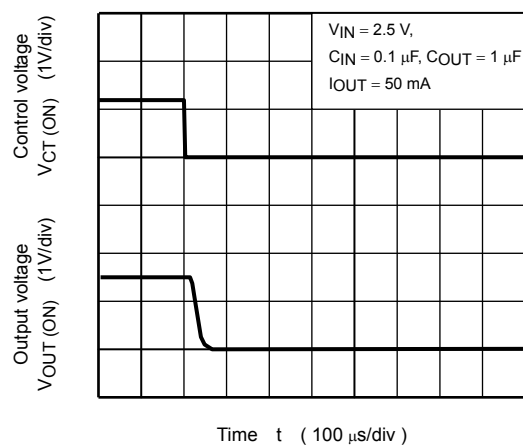
TCR5SB15A (Turn off wave form)
