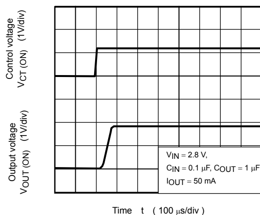
TCR5SB18A (Turn on wave form)
