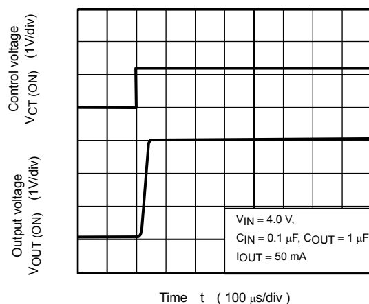
TCR5SB30A (Turn on wave form)
