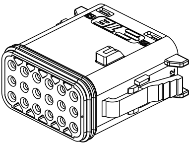
18CCT PLUG CONNECTOR WITHOUT HEATSHRINK HOUSING
