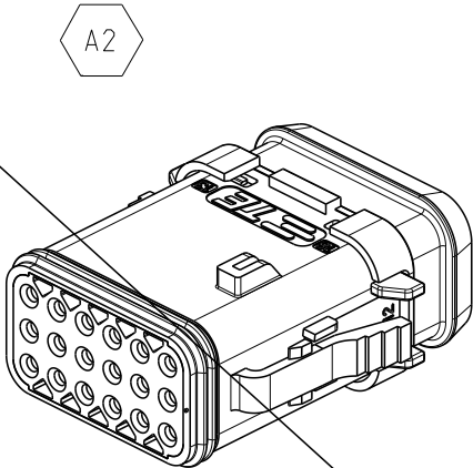
18CCT PLUG CONNECTOR WITH HEATSHRINK HOUSING
