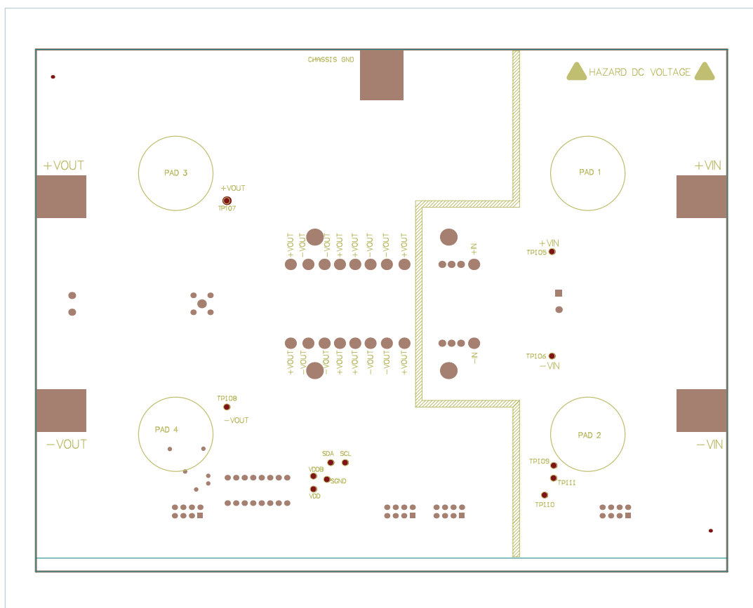
Figure 6 BPCB#42030 Evaluation Board
