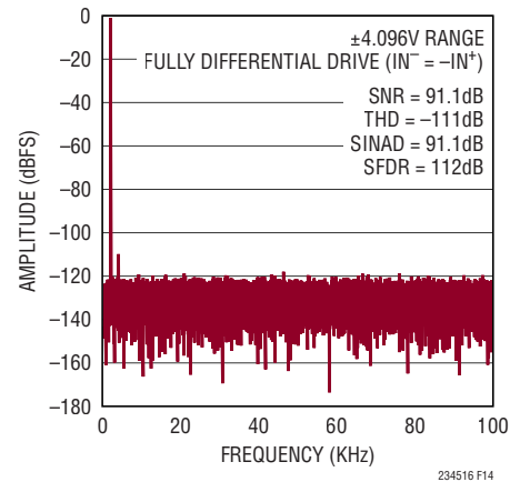
Figure 14. 32k Point FFT f_{\text{SMPL}} = 200\text{ksps} , f_{\text{IN}} = 2\text{kHz}
