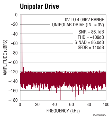
Figure 6e. IN^+ = -1\text{dBFS} 2kHz Unipolar Sine, IN^- = 0\text{V} , 32k Point FFT, f_{\text{SAMPL}} = 200\text{kpsps} . Circuit Shown in Figure 6a with LT6237 Amplifiers, R_{\text{FILT}} = 40.2\Omega , C_{\text{FILT}} = 1\text{nF}
