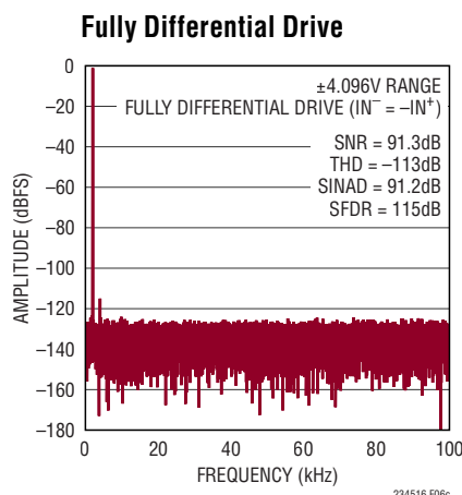
Figure 6c. IN^+/IN^- = -1\text{dBFS} 2kHz Fully Differential Sine, Common Mode = 2.5V, 32k Point FFT, f_{\text{SAMPL}} = 200\text{kpsps} . Circuit Shown in Figure 6a with LT6237 Amplifiers, R_{\text{FILT}} = 40.2\Omega , C_{\text{FILT}} = 1\text{nF}
