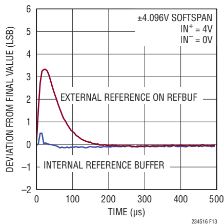
Figure 13. Burst Conversion Response of the LTC2345-16, f_{\text{SMPL}} = 200\text{ksps}
