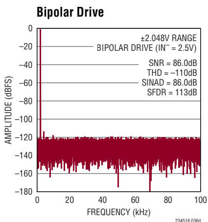
Figure 6d. IN^+ = -1\text{dBFS} 2kHz Bipolar Sine, IN^- = 2.5\text{V} , 32k Point FFT, f_{\text{SAMPL}} = 200\text{kpsps} . Circuit Shown in Figure 6a with LT6237 Amplifiers, R_{\text{FILT}} = 40.2\Omega , C_{\text{FILT}} = 1\text{nF}
