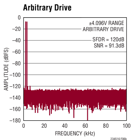
Figure 6b. Two-Tone Test. IN^+ = -7\text{dBFS} 2kHz Sine, IN^- = -7\text{dBFS} 3.1kHz Sine, Common Mode = 2.5V, 32k Point FFT, f_{\text{SAMPL}} = 200\text{kpsps} . Circuit Shown in Figure 6a with LT6237 Amplifiers, R_{\text{FILT}} = 40.2\Omega , C_{\text{FILT}} = 1\text{nF}
