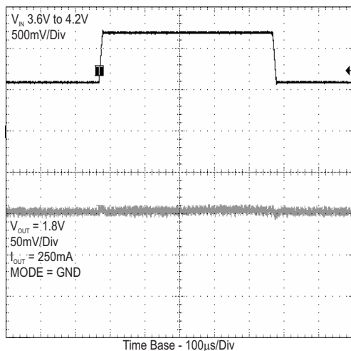
Figure 25. PFM Line Transient
