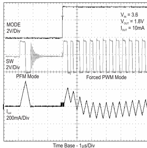
Figure 26. Mode Transition PFM to PWM
