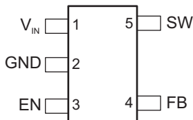
DDC Package 5-Pin SOT Top View
