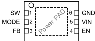
Pin Functions
