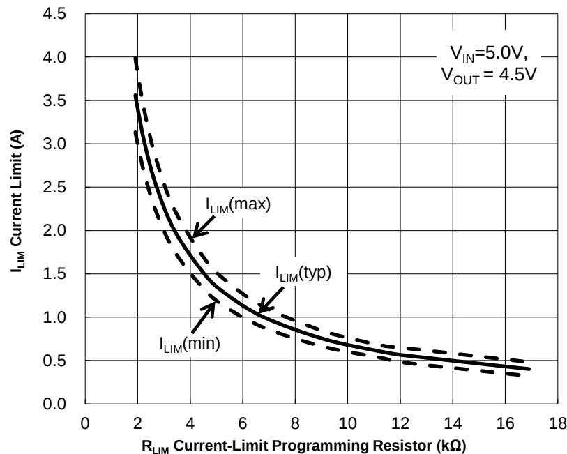
Figure 2. R_{LIMIT} vs. Overload Current Limit
