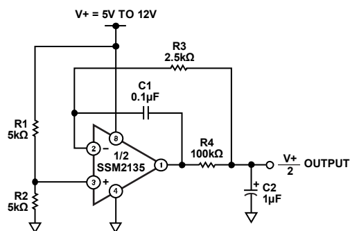
Figure 37. Pseudoreference Generator
