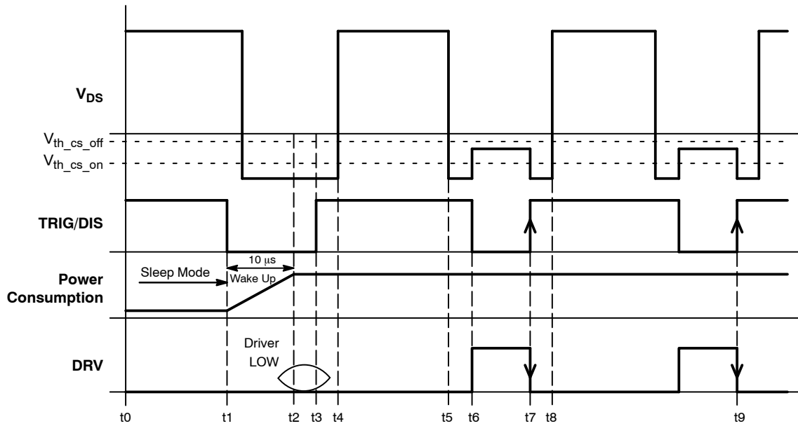
Figure 57. Waking-up Sequence
