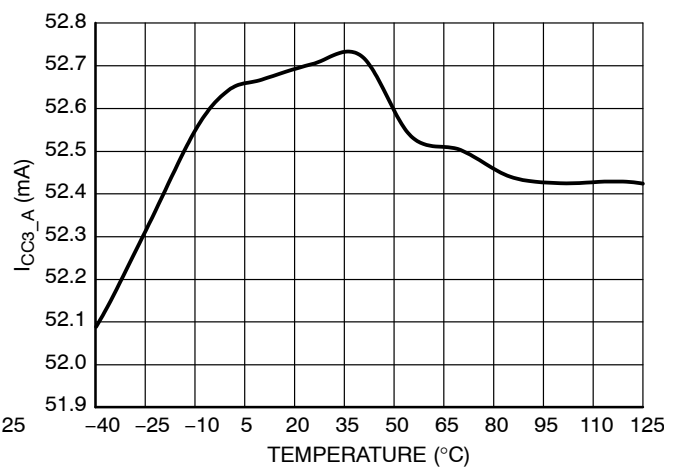
Figure 38. Internal IC Consumption (A Version, C_{DRV} = 10 \text{ nF} , f_{SW} = 400 \text{ kHz} , t_{on\_min} = 500 \text{ ns} , t_{off\_min} = 620 \text{ ns} )
