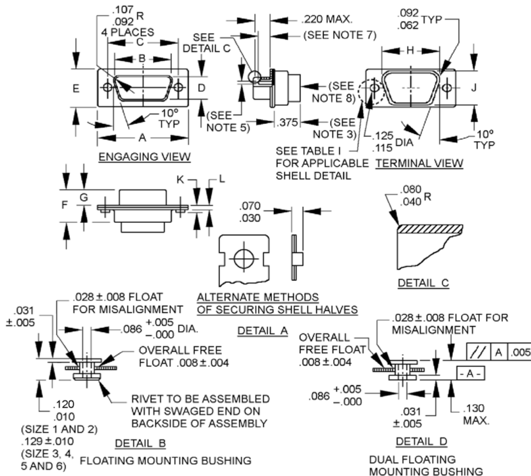
FIGURE 1. Shell, plug, crimp type.
