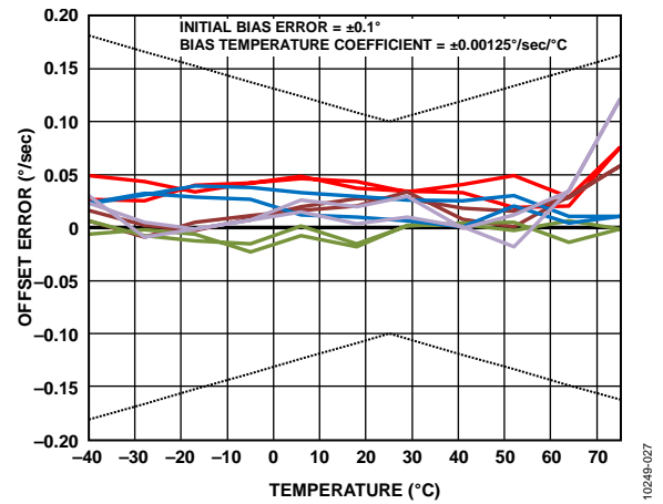
Figure 9. Offset (Bias) Error vs. Temperature, -40^\circ\text{C} to +75^\circ\text{C} to -40^\circ\text{C}
