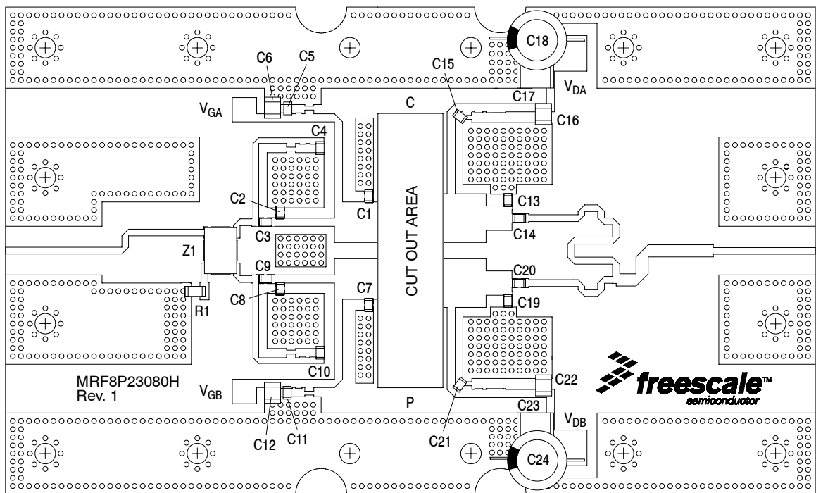
Figure 2. MRF8P23080HR3(HSR3) Test Circuit Component Layout
