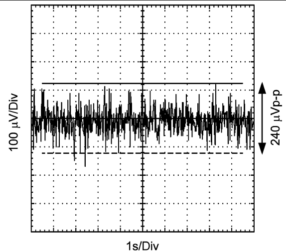
Figure 26. 0.1–10 Hz Noise
