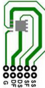
b) 116 ^{\circ}\text{C}/\text{W} when mounted on a minimum pad of 2 oz copper.
