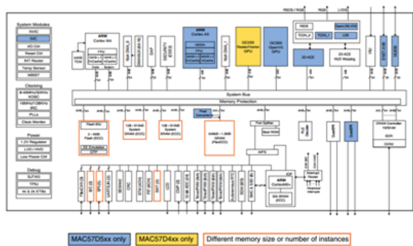
Figure 1. Block diagram
