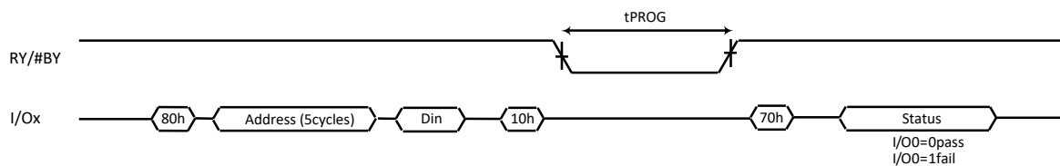
Figure 9-9 Page Program
