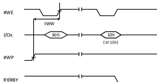
Figure 9-24 Program Enable
