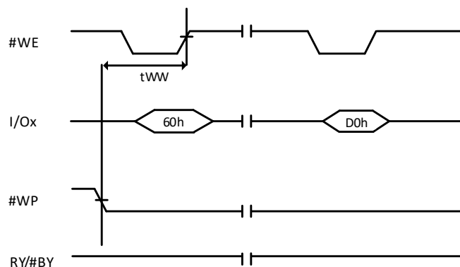
Figure 9-23 Erase Disable
