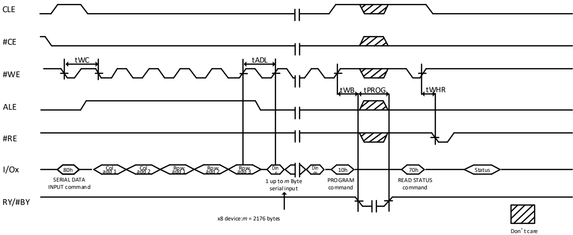
Figure 11-11 Page Program
