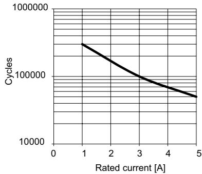
AC 15, Ue=250Vac, +23°C Typical electrical endurance (load acc. IEC 60947-5-1, evaluation acc. IEC 61810-2)
