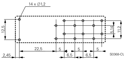
4 form A + 2 form B, 4 NO + 2 NC versions SR6
