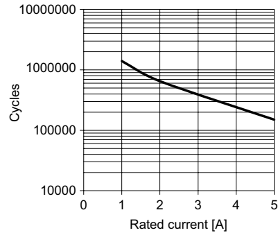
DC 13, Ue=24Vdc, +23°C Typical electrical endurance (load acc. IEC 60947-5-1, evaluation acc. IEC 61810-2)
