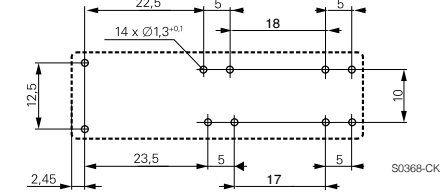
3 form A + 1 form B, 3 NO + 1 NC contacts
