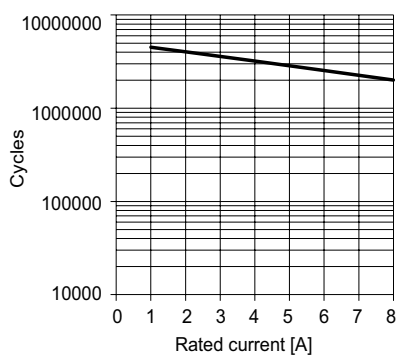
DC resistive, Ue=24Vdc, +23°C Typical electrical endurance (load acc. IEC 61810-1, evaluation acc. IEC 61810-2)
