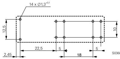
2 form A + 2 form B, 2 NO + 2 NC versions
