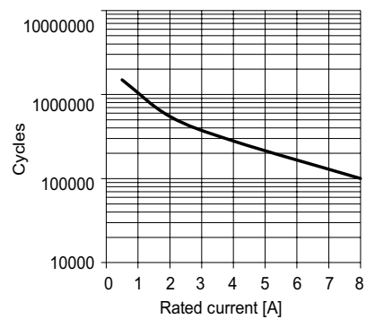
AC resistive, Ue=250Vac, +85°C Typical electrical endurance (load acc. IEC 61810-1, evaluation acc. IEC 61810-2)
