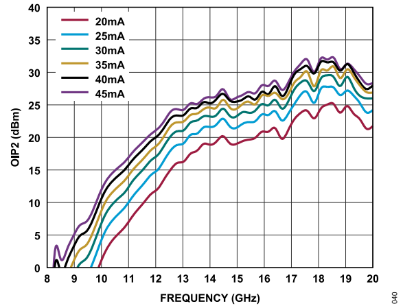
Figure 40. OIP2 vs. Frequency for Various I_{DQ} , V_{DD} = 1.5 V
