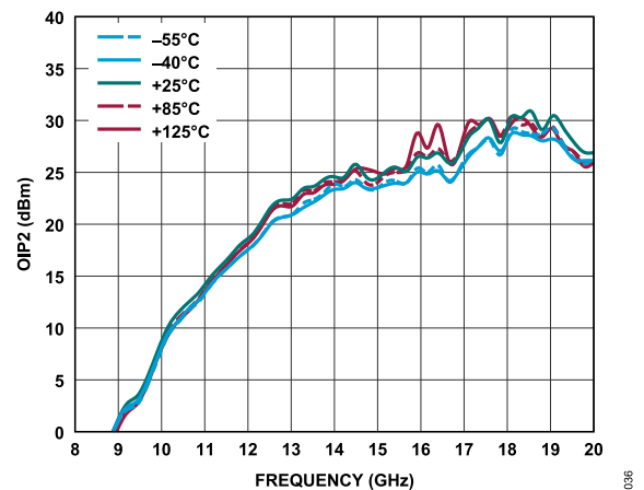
Figure 36. OIP2 vs. Frequency for Various Temperatures, V_{DD} = 1.5 V, I_{DQ} = 35 mA, and R_{BIAS} = 562 \Omega
