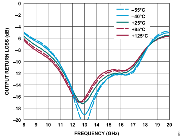
Figure 16. Output Return Loss vs. Frequency for Various Temperatures, V_{DD} = 1.5 V, I_{DQ} = 35 mA, and R_{BIAS} = 562 \Omega
