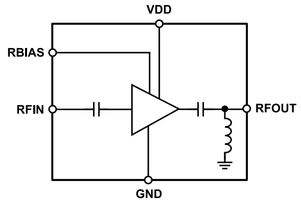
Figure 49. Simplified Schematic
