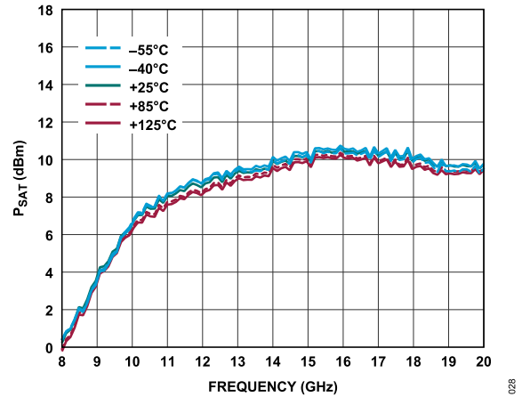
Figure 28. P_{SAT} vs. Frequency for Various Temperatures, V_{DD} = 1.5 V, I_{DQ} = 35 mA, and R_{BIAS} = 562 \Omega
