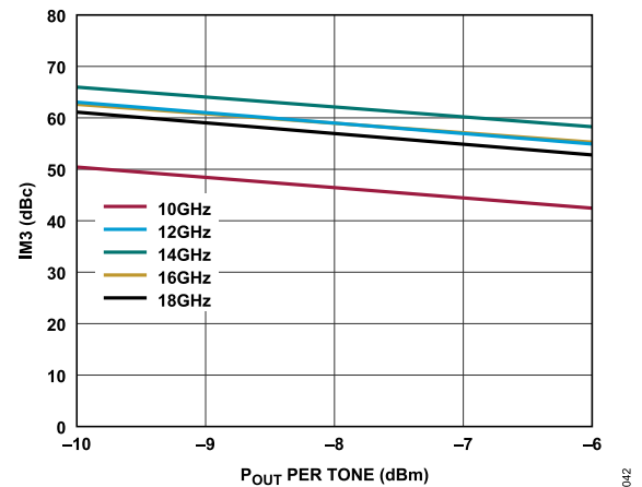
Figure 42. Third-Order Intermodulation (IM3) vs. P_{OUT} per Tone for Various Frequencies, V_{DD} = 1.5 V and R_{BIAS} = 562 \Omega
