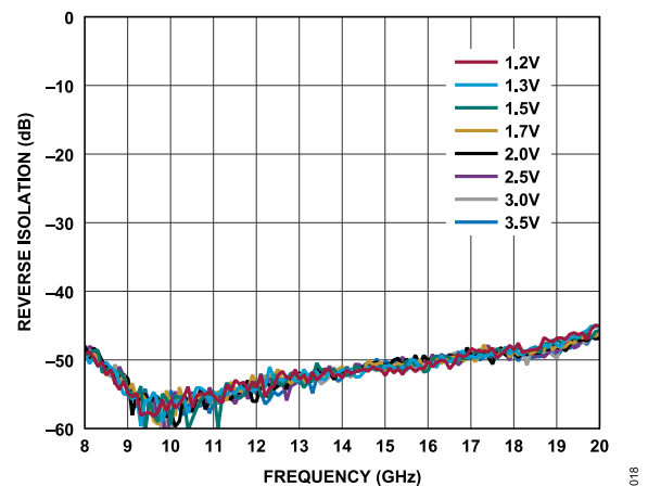
Figure 18. Reverse Isolation vs. Frequency for Various Supply Voltages, I_{DQ} = 35 mA
