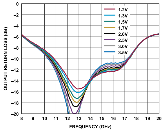
Figure 14. Output Return Loss vs. Frequency for Various Supply Voltages, I_{DQ} = 35 mA
