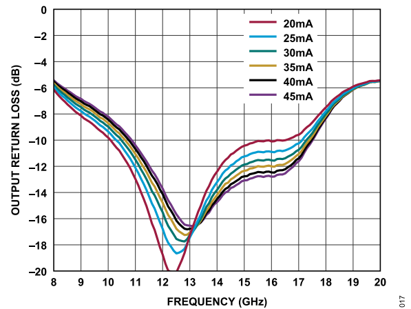
Figure 17. Output Return Loss vs. Frequency for Various I_{DQ} , V_{DD} = 1.5 V
