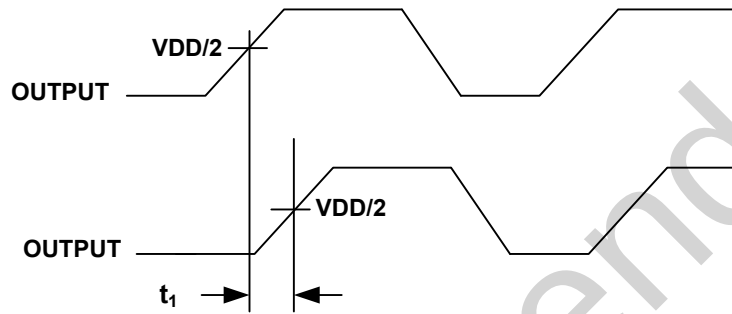
Figure 2. Output to Output Skew
