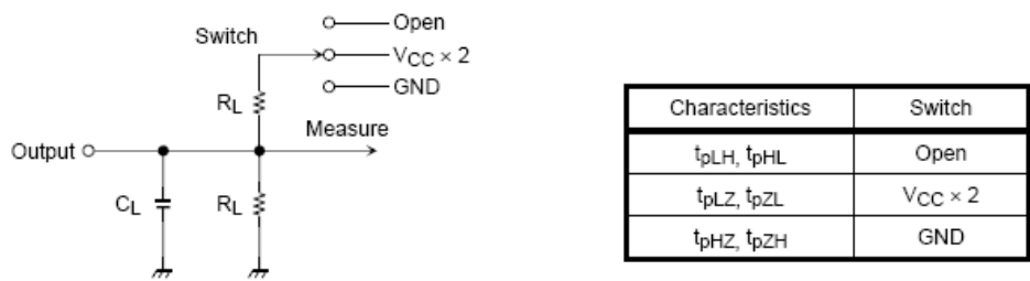
Figure 3. Test Circuit
