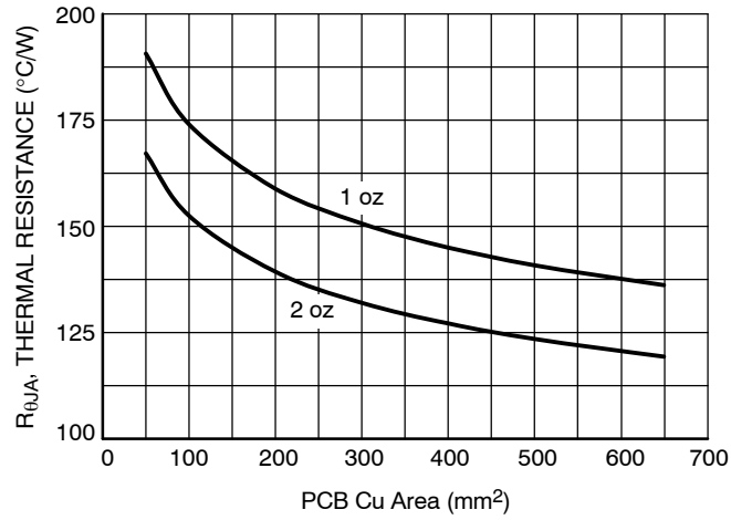
Figure 18. R_{\theta JA} vs. PCB Cu Area
