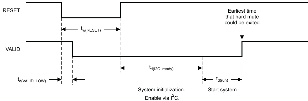
Figure 4. Reset Timing
