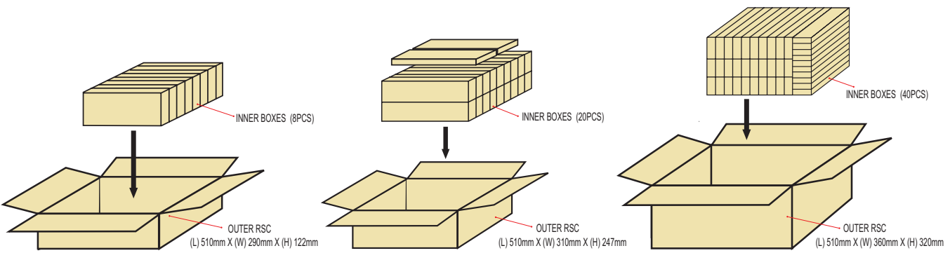
Figure 13. Dimensions for outer box packaging for LUXEON CoB (Gen2).
