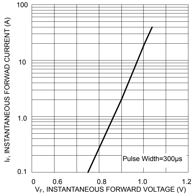
Fig.2 Typical Fwd Characteristics, per element
