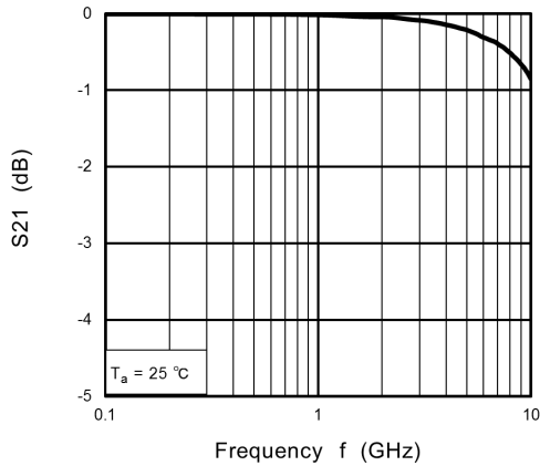
Fig. 9.5 S_{21} - f
