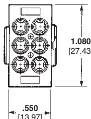
Cap Rear
