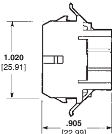
Cap Front
