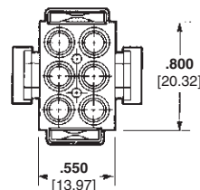
Plug Front
