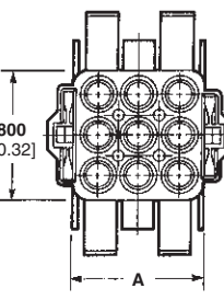
Cap Front
