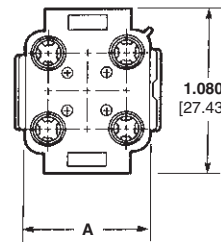
Plug Front
