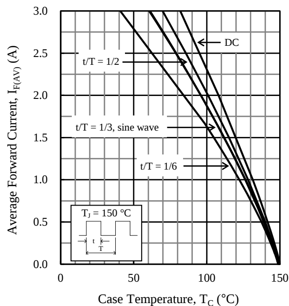
Figure 2. Typical Characteristics: I_{F(AV)} vs. T_C ( V_R = 500 V)
