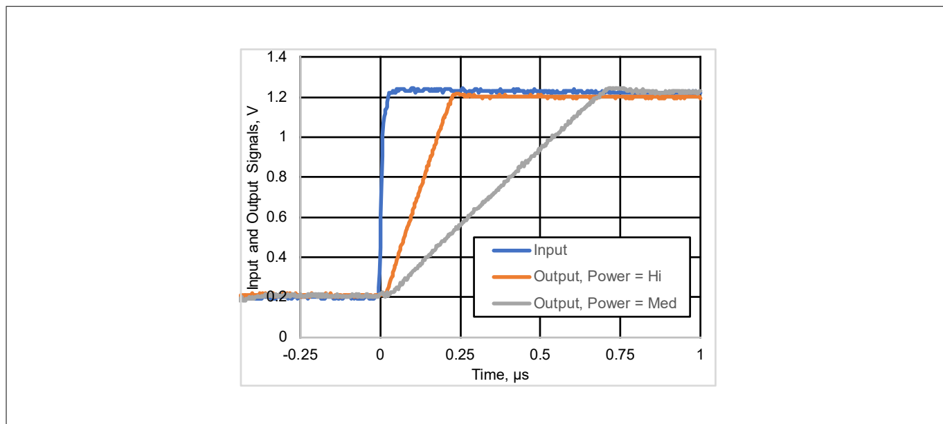
Figure 17 Opamp step response, rising
