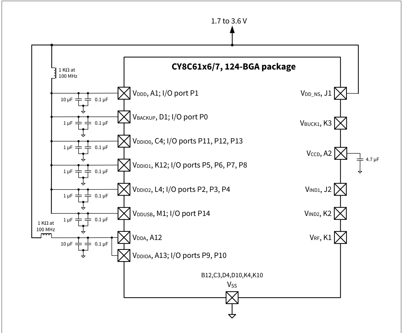
Figure 12 124-BGA (No buck) power connection diagram
