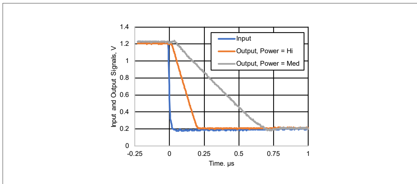
Figure 18 Opamp step response, falling
