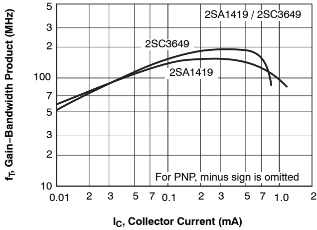
Figure 10. f_T - I_C
