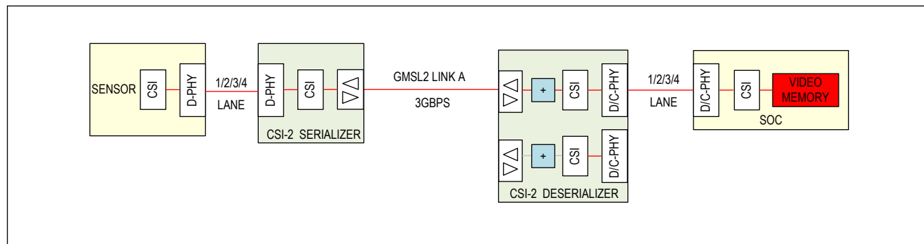
Figure 13. Single Link
