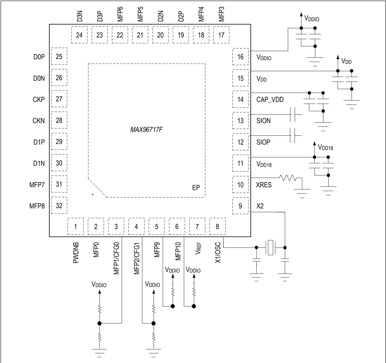
Typical Application Circuit
