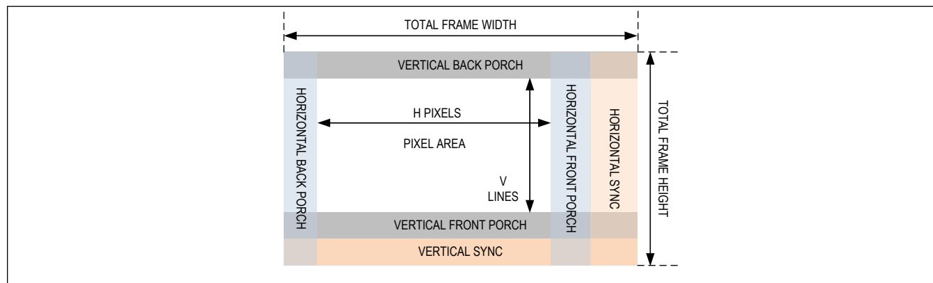
Figure 28. Video Timing
