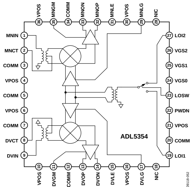
Figure 51. Simplified Schematic
