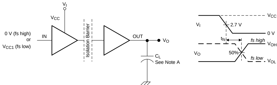
Figure 13. Failsafe Delay Time Test Circuit and Voltage Waveforms
