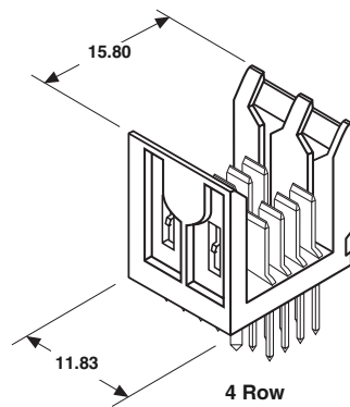
4 Row
