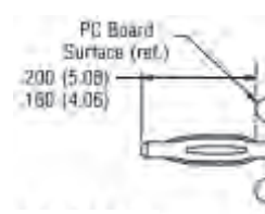
Press-fit Tail Detail
