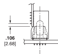
Mating Condition
