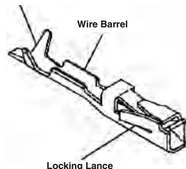
Locking Lance
