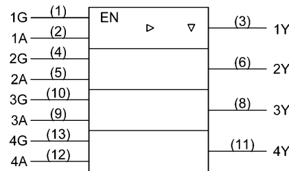
74VHCT126AFT
