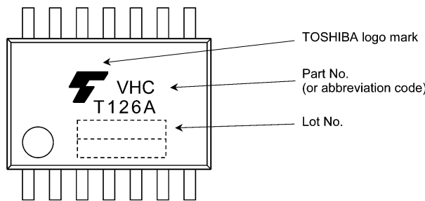
74VHCT126AFT
