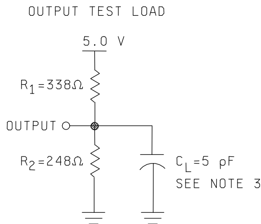
Circuit A or equivalent ( t_{EA} and t_{ER} )
