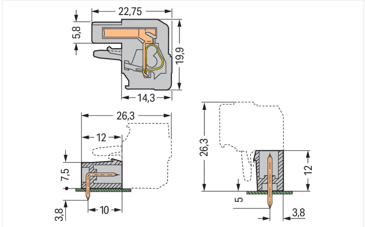
Dimensions in mm L = (pole no. x pin spacing) + 1.5 mm + 0.9 mm 2- to 3-pole female connectors – one latch only
