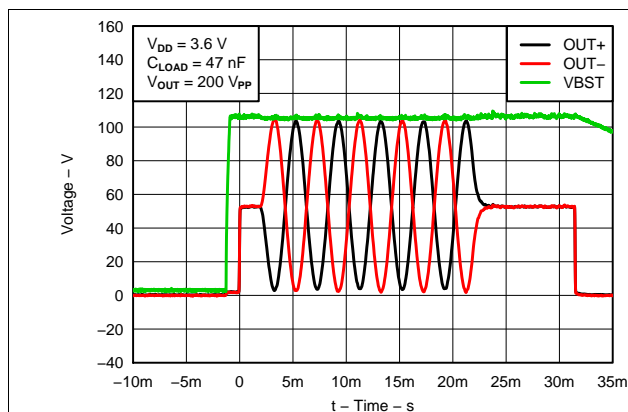
Figure 15. Typical Waveform
