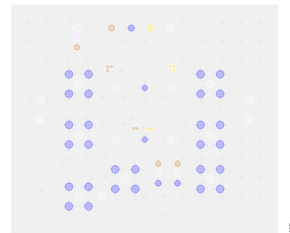
Figure 7. EVAL-ADG7421FEBZ Layer 2
