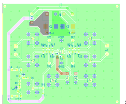
Figure 6. EVAL-ADG7421FEBZ Top Layer
