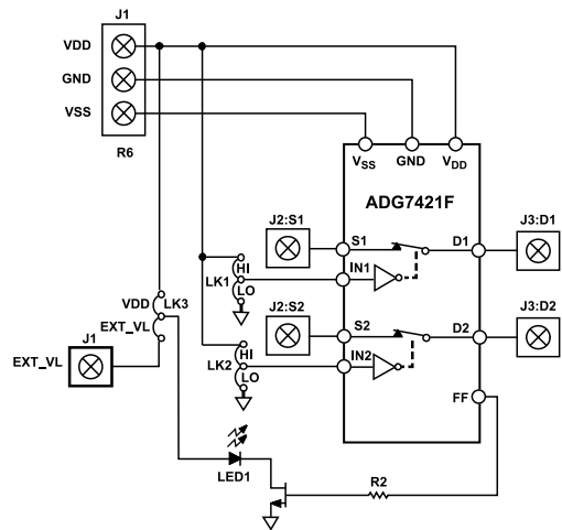
Figure 2. EVAL-ADG7421FEBZ Block Diagram
