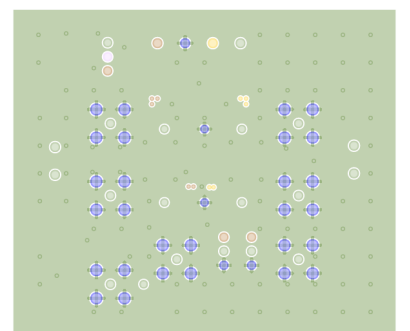
Figure 8. EVAL-ADG7421FEBZ Layer 3
