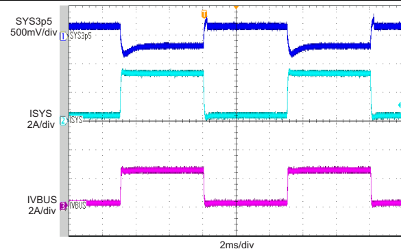
Figure 43. PWM Switching in Buck Mode
